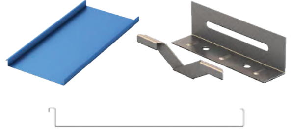
CLIP | DMC 150SS BUTTERFLY
